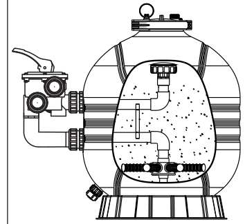
TYPICAL INSTALLATION
