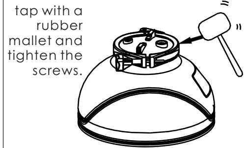
FIGURE3.-Clamp Installation
