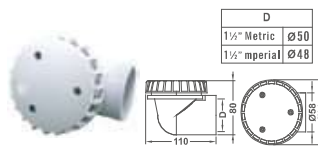
φ2 Section Drain Ell Body(Threaded)
