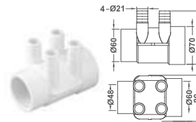
Port Water Barb Manifold
