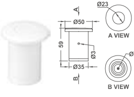
Air Button
