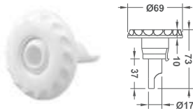
φ2-3/4" Vortex Face Eyeball Spa Jet
