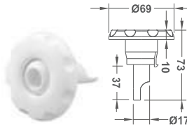
φ2-3/4" Face Eyeball Spa Jet
