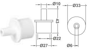
Barb Plug
