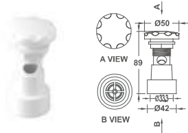
φ25mm Air Control
