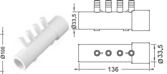
Port Air Manifold
