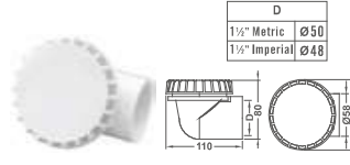
φ2 Section Drain Ell Body(Slip Fit)
