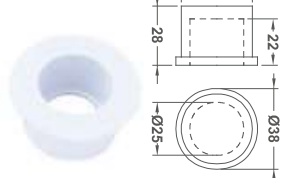
Pipe Plug
