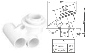
φ25mm Barb Air & φ25mm Water Tee Body
