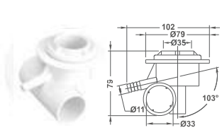
φ10mm Barb Air & φ25mm Water
