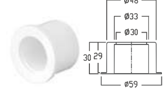
Pipe Plug
